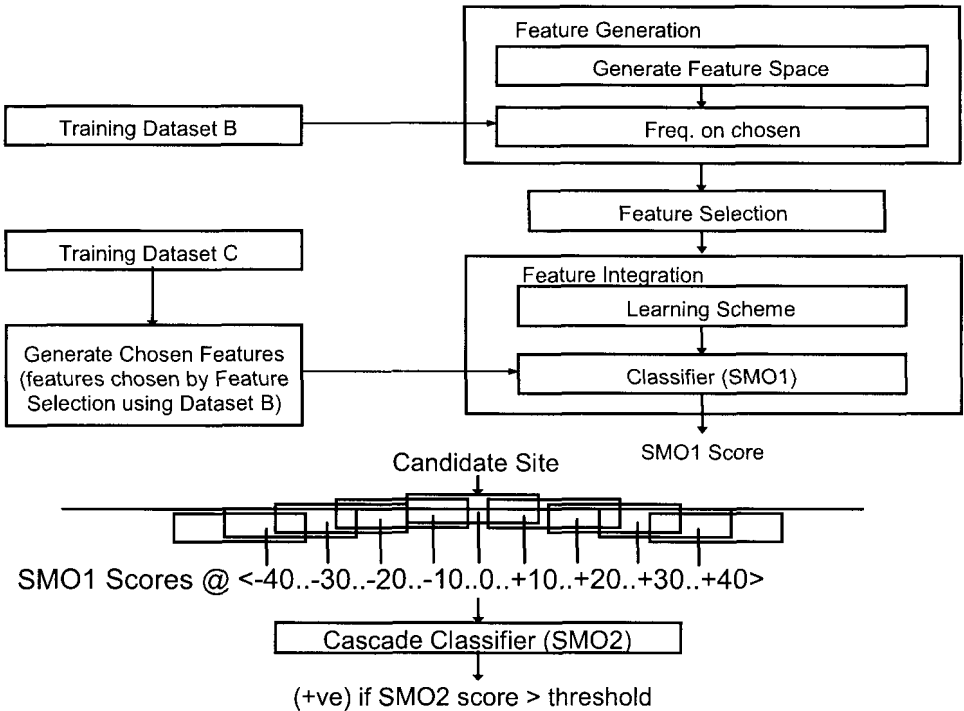
Figure 2. Architecture of our polyadenylation prediction system.
